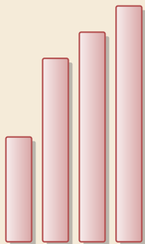
run2
